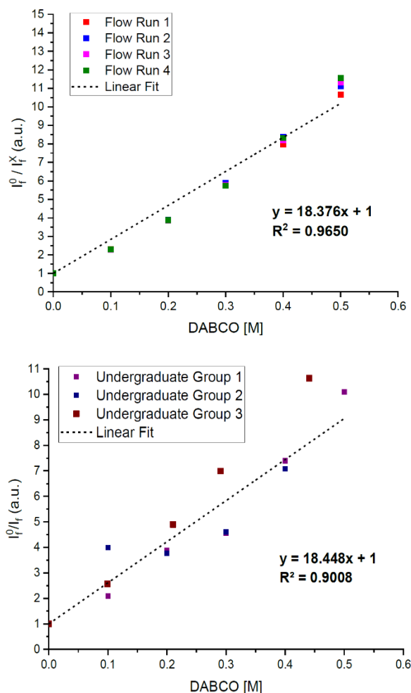
Figure 5 - Results of the Stern-Volmer fluorescence quenching analysis (A) performed using the PS-2600 and flow system (B) Performed by three, independent groups of undergraduate students using a commercial fluorimeter
